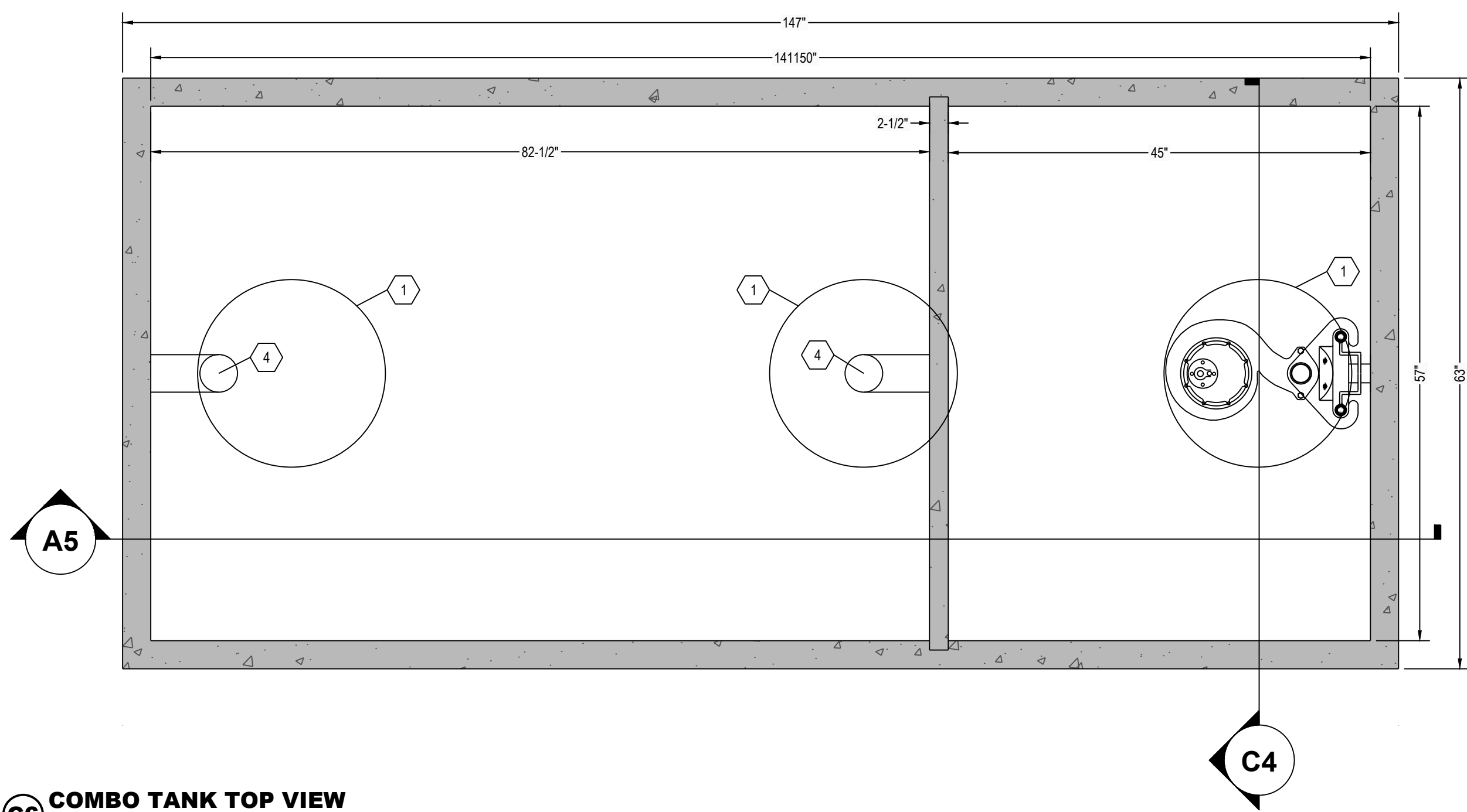
C6 COMBO TANK TOP VIEW 1" = 1"
