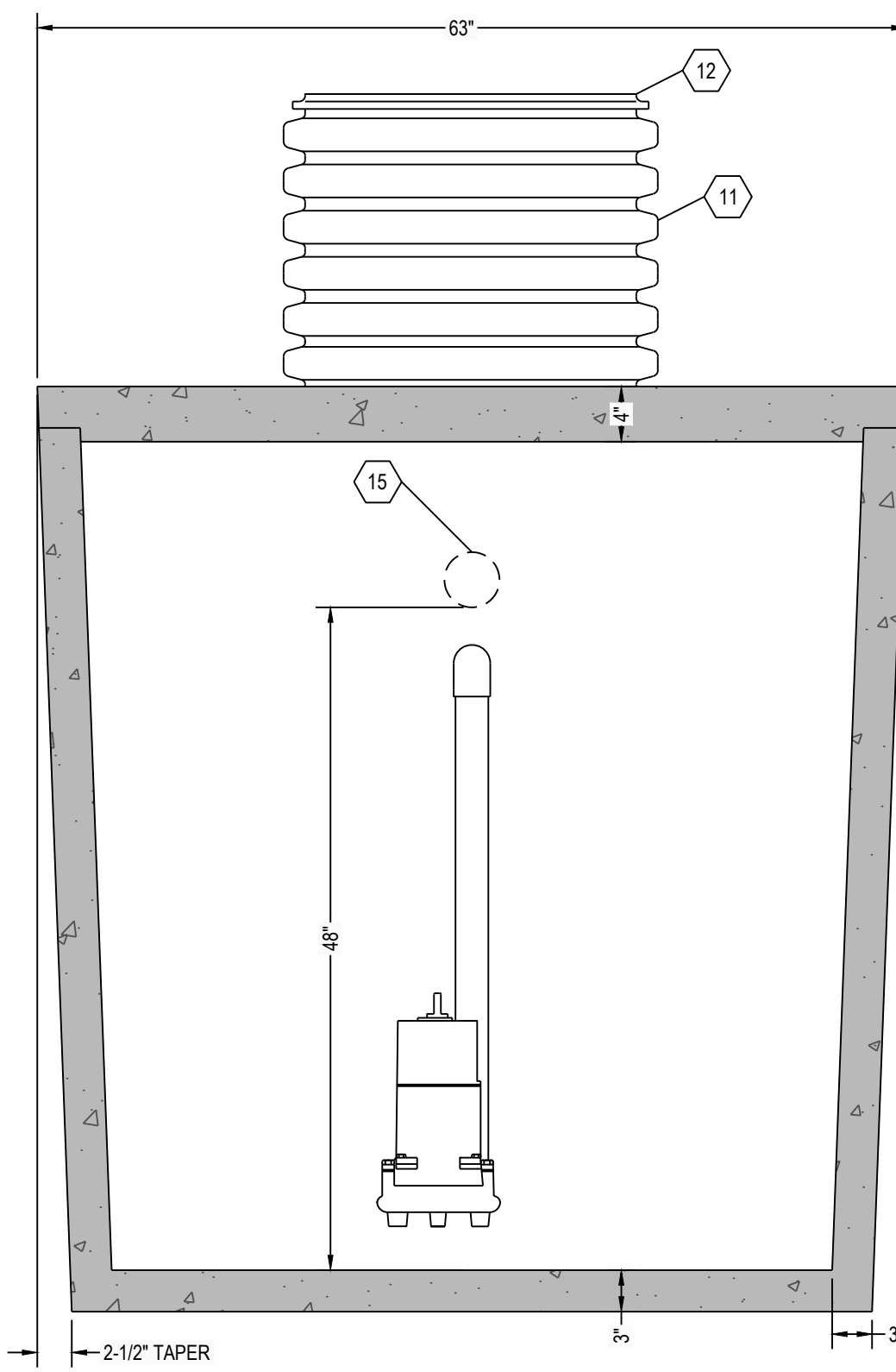
C4 COMBO TANK SECTION VIEW 1" = 1"
